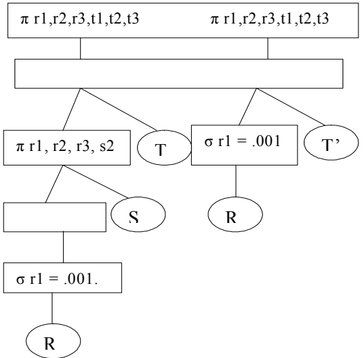
Figure 10. Comparison Using Query Trees
